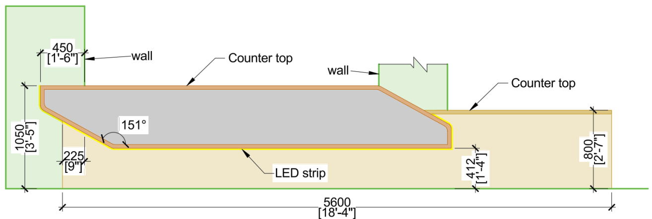
COUNTER FRONT VIEW
