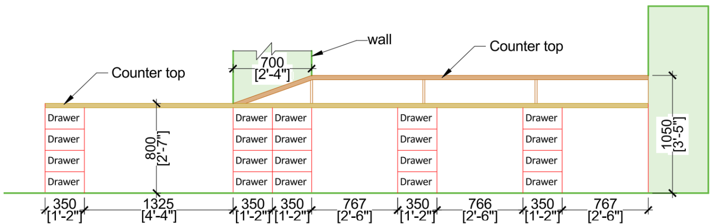
COUNTER INTERIOR SIDE VIEW
